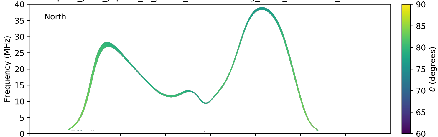
expres_juno_jupiter_io_jrm09_lossc-wid1deg_3kev_20190625_v01.cdf
