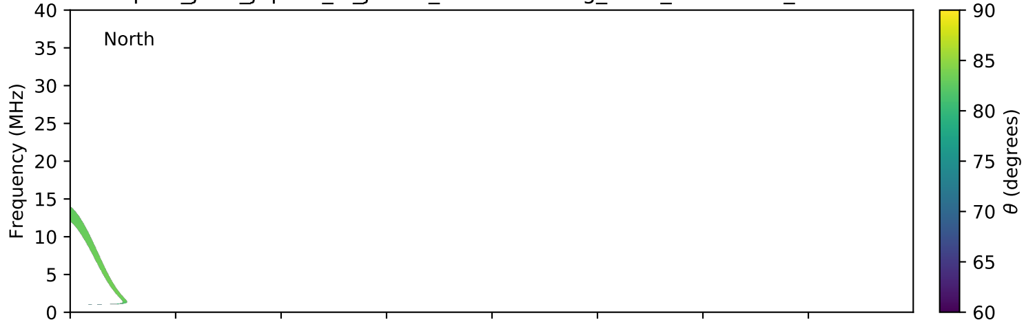
expres_juno_jupiter_io_jrm09_lossc-wid1deg_3kev_20190624_v01.cdf
