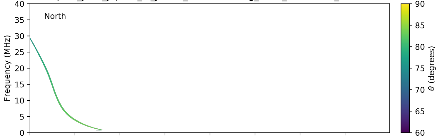
expres_juno_jupiter_io_jrm09_lossc-wid1deg_3kev_20190622_v01.cdf
