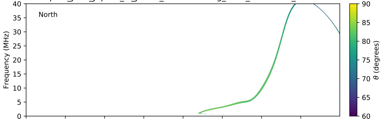
expres_juno_jupiter_io_jrm09_lossc-wid1deg_3kev_20190621_v01.cdf
