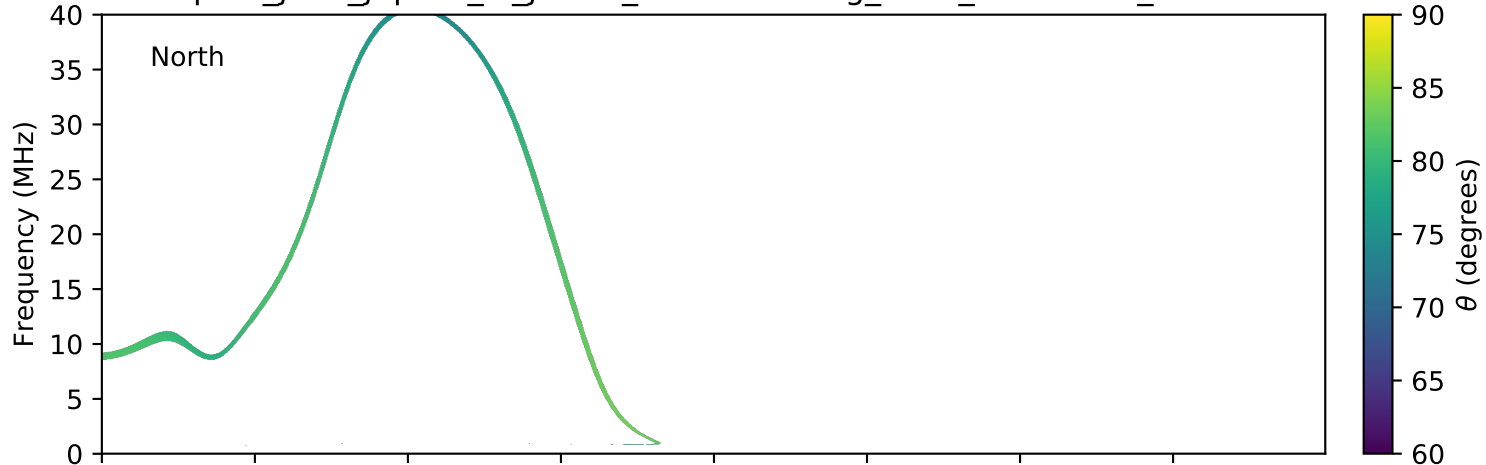
expres_juno_jupiter_io_jrm09_lossc-wid1deg_3kev_20190620_v01.cdf
