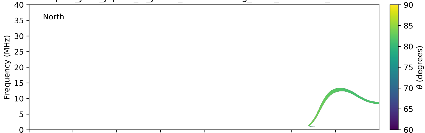
expres_juno_jupiter_io_jrm09_lossc-wid1deg_3kev_20190619_v01.cdf
