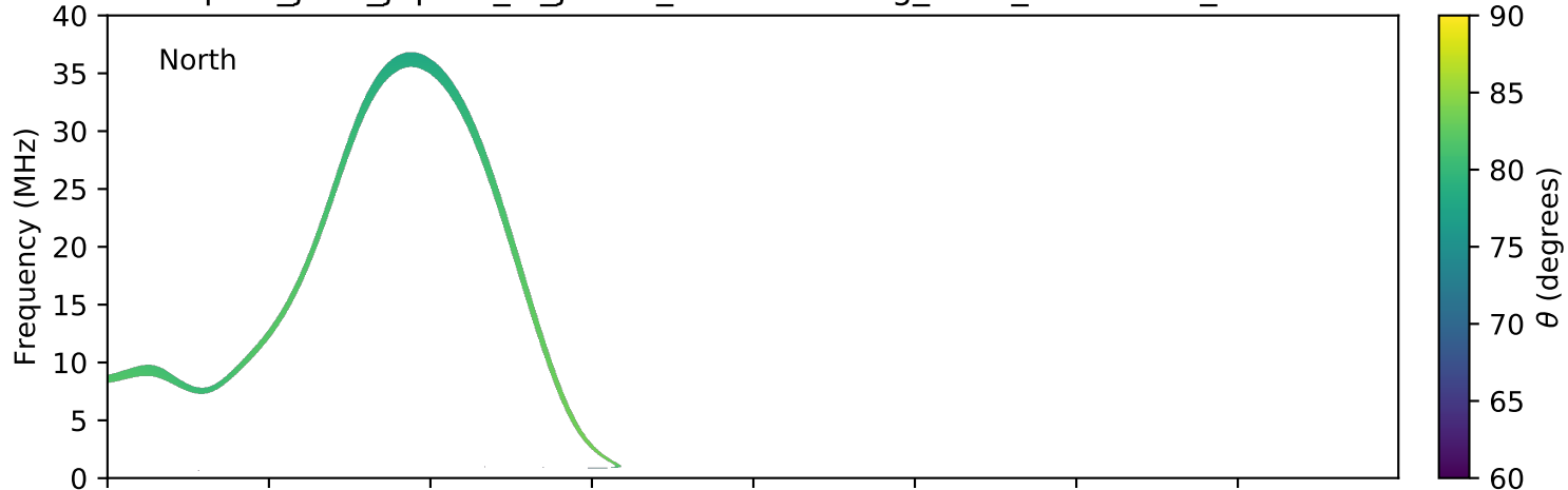
expres_juno_jupiter_io_jrm09_lossc-wid1deg_3kev_20190613_v01.cdf
