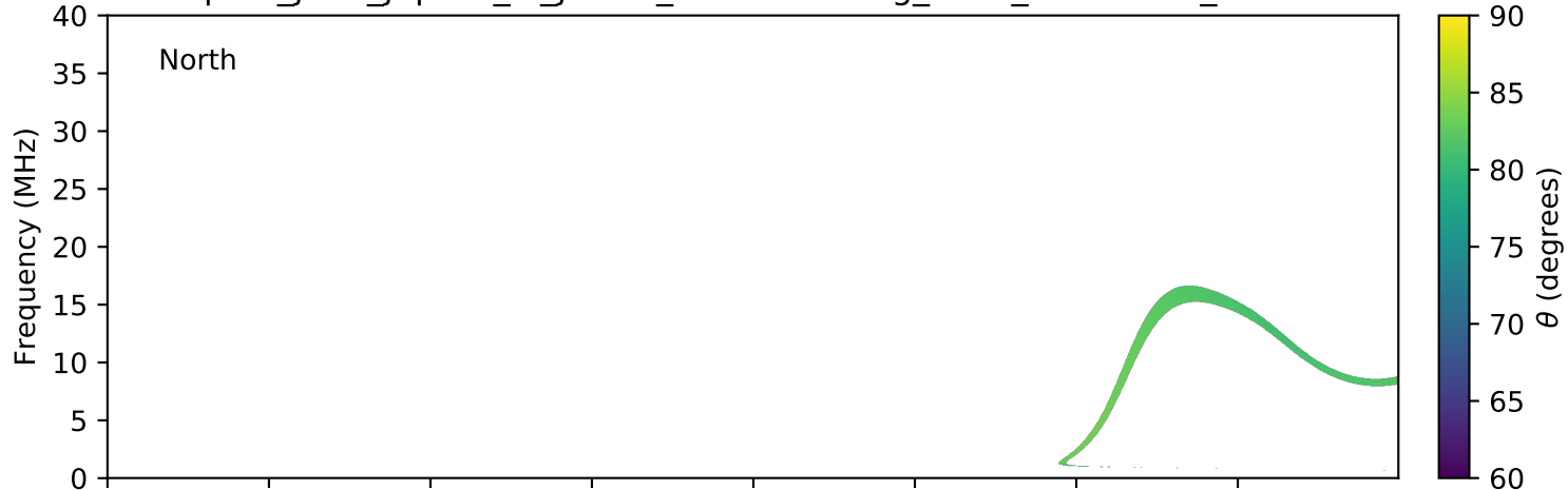
expres_juno_jupiter_io_jrm09_lossc-wid1deg_3kev_20190612_v01.cdf
