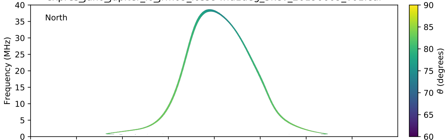
expres_juno_jupiter_io_jrm09_lossc-wid1deg_3kev_20190609_v01.cdf
