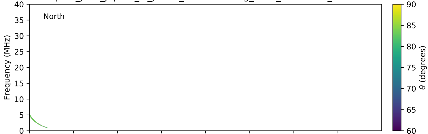
expres_juno_jupiter_io_jrm09_lossc-wid1deg_3kev_20190608_v01.cdf
