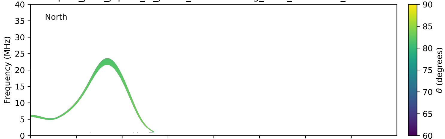
expres_juno_jupiter_io_jrm09_lossc-wid1deg_3kev_20190606_v01.cdf
