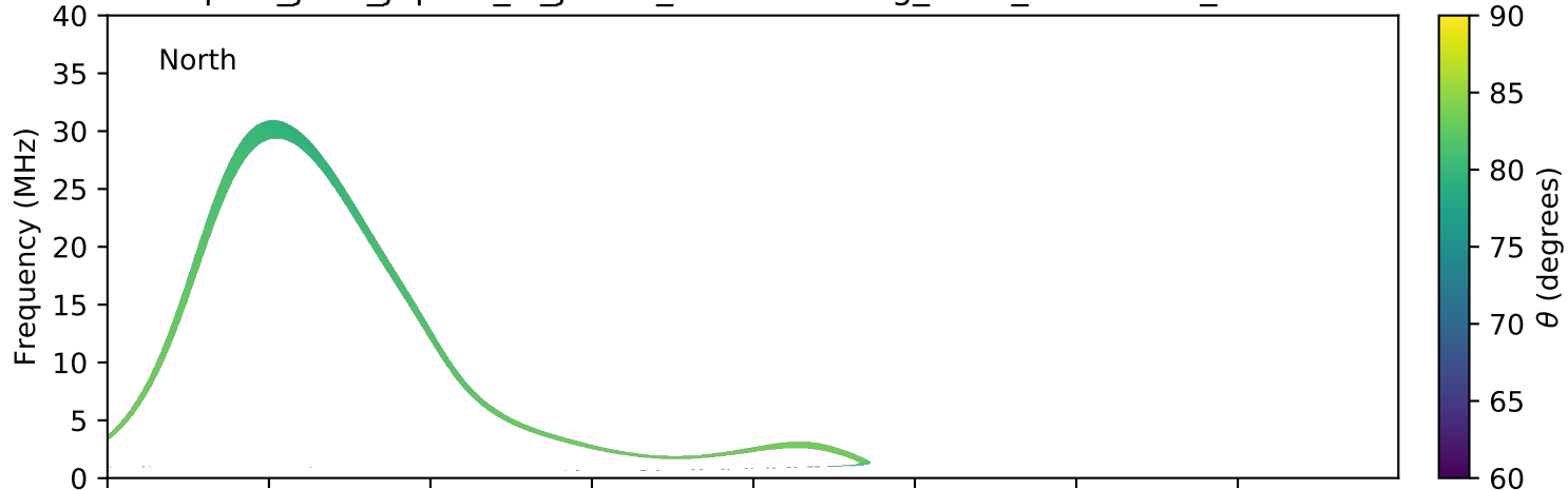
expres_juno_jupiter_io_jrm09_lossc-wid1deg_3kev_20190604_v01.cdf
