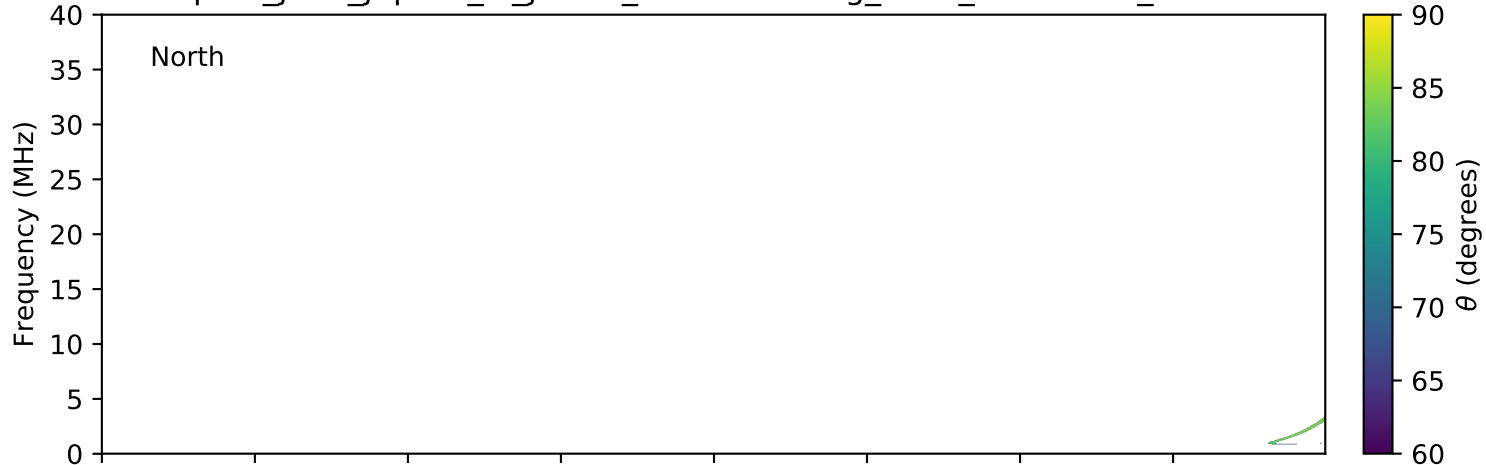
expres_juno_jupiter_io_jrm09_lossc-wid1deg_3kev_20190603_v01.cdf
