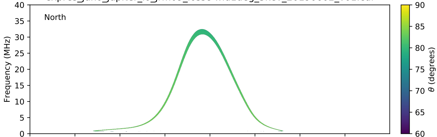
expres_juno_jupiter_io_jrm09_lossc-wid1deg_3kev_20190602_v01.cdf
