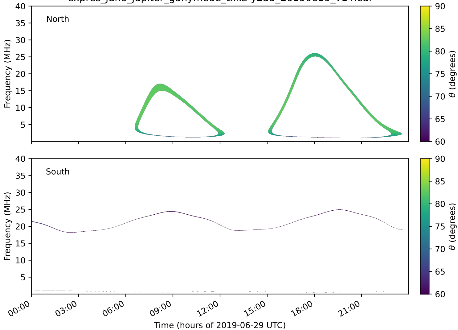
expres_juno_jupiter_ganymede_txka-y235_20190629_v14.cdf
