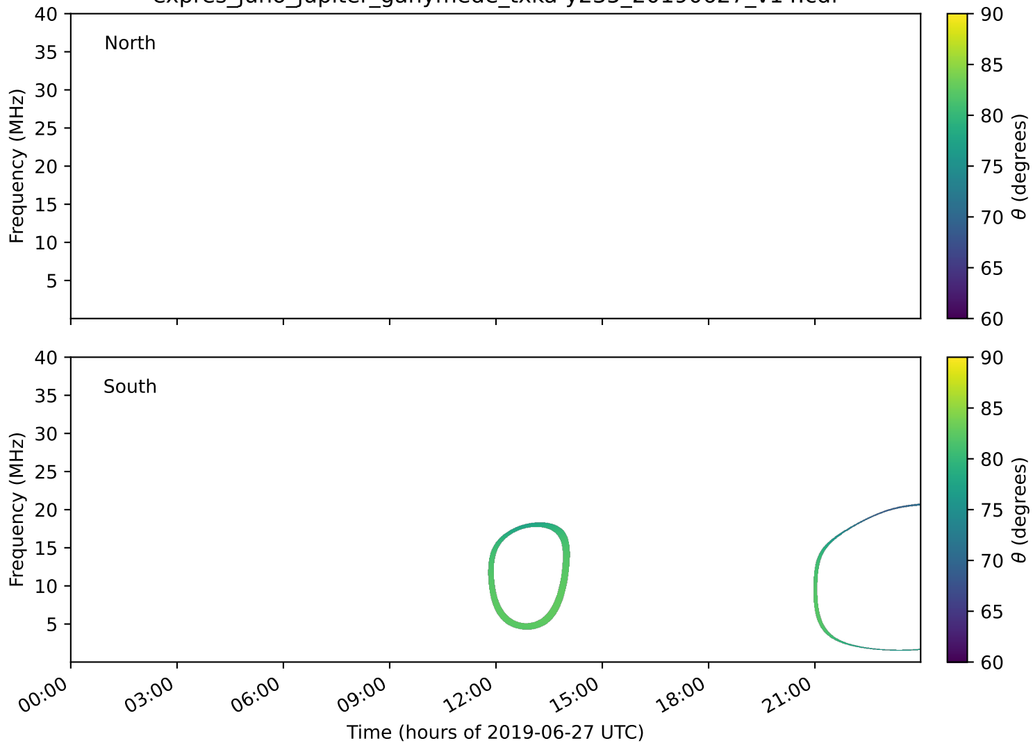
expres_juno_jupiter_ganymede_txka-y235_20190627_v14.cdf
