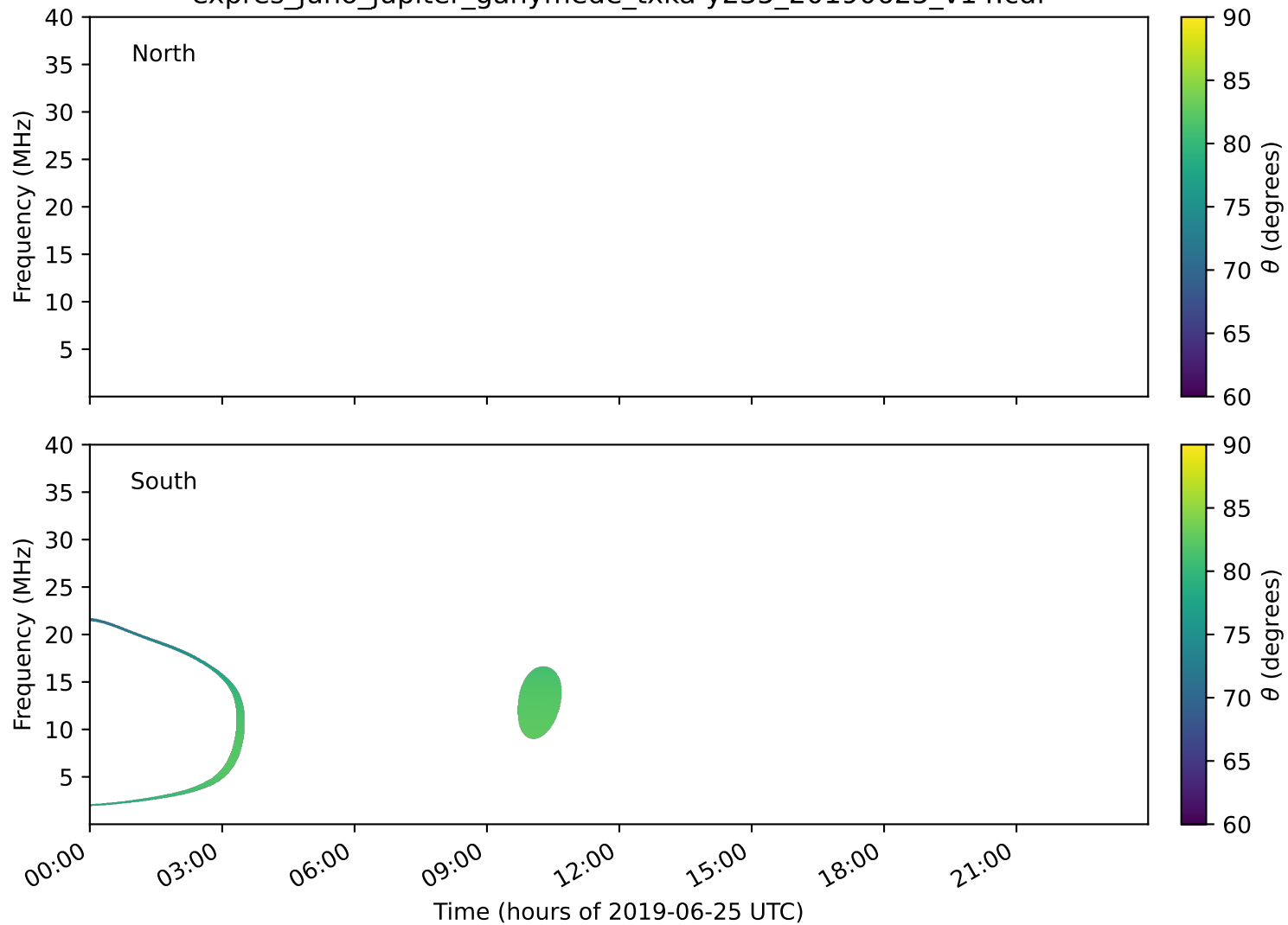
expres_juno_jupiter_ganymede_txka-y235_20190625_v14.cdf
