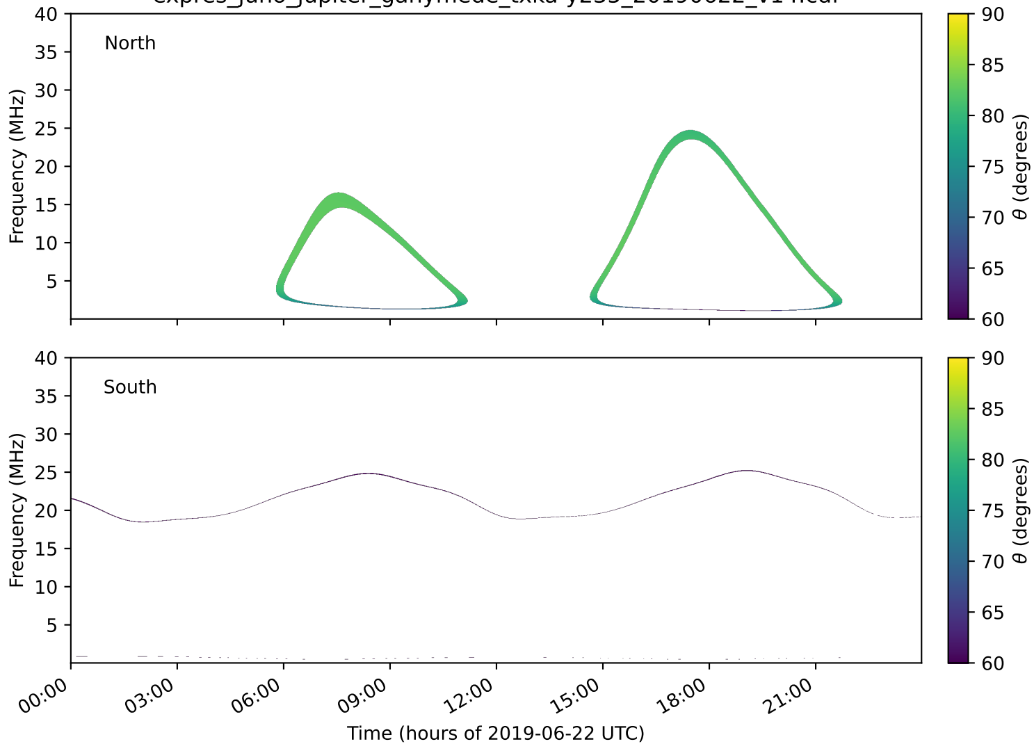
expres_juno_jupiter_ganymede_txka-y235_20190622_v14.cdf
