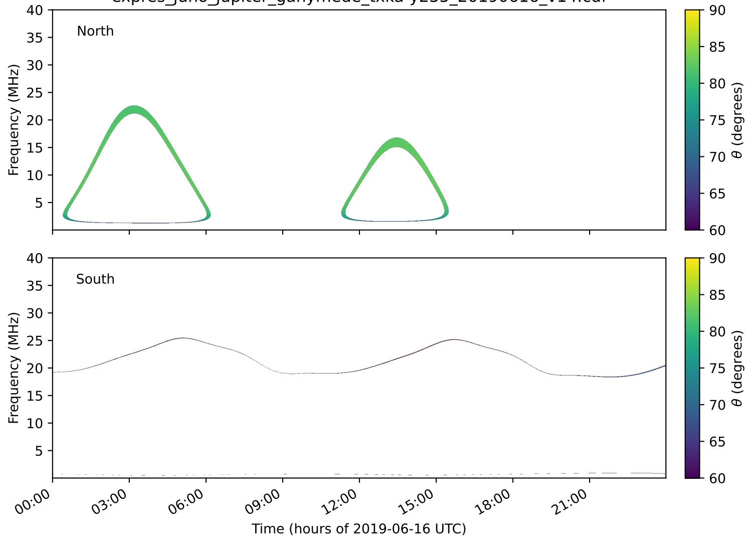
expres_juno_jupiter_ganymede_txka-y235_20190616_v14.cdf
