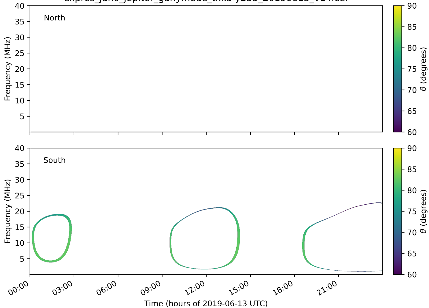
expres_juno_jupiter_ganymede_txka-y235_20190613_v14.cdf
