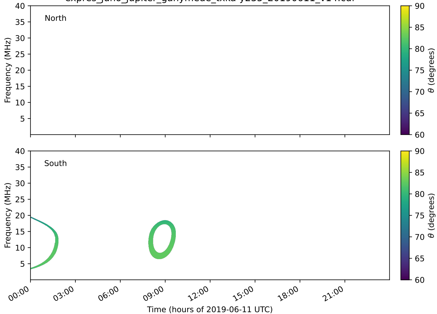
expres_juno_jupiter_ganymede_txka-y235_20190611_v14.cdf
