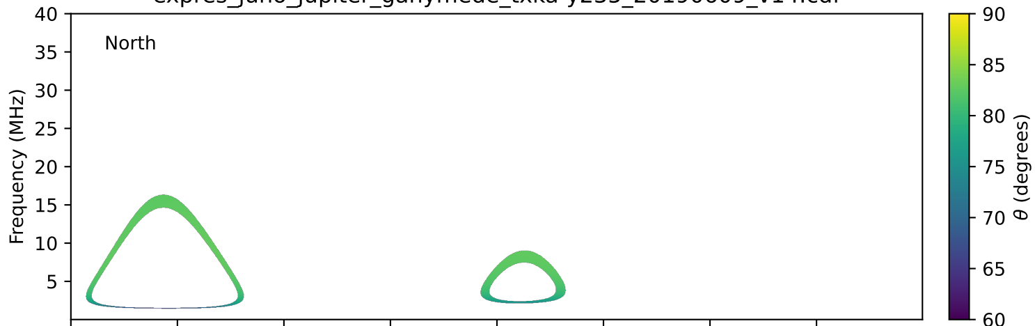
expres_juno_jupiter_ganymede_txka-y235_20190609_v14.cdf
