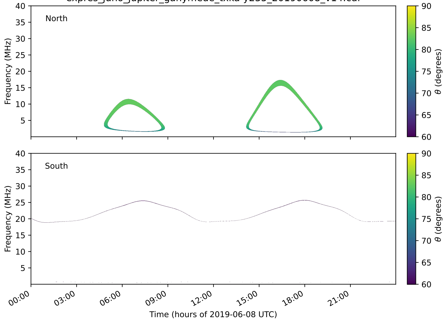
expres_juno_jupiter_ganymede_txka-y235_20190608_v14.cdf
