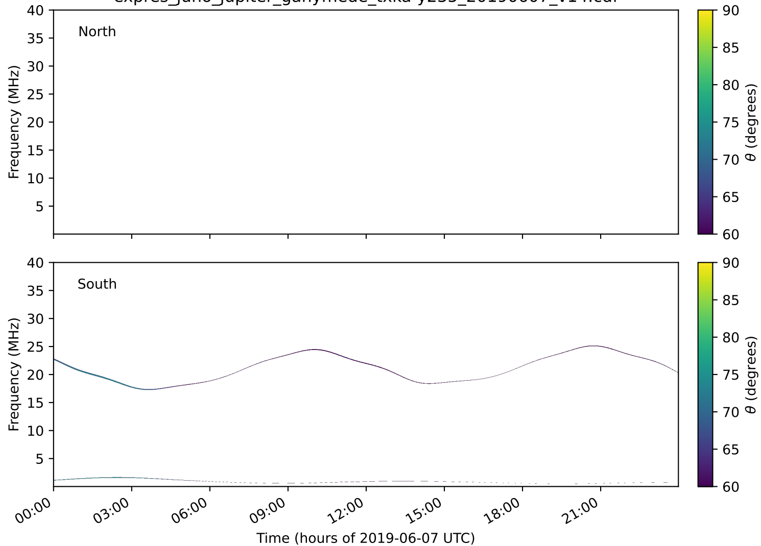
expres_juno_jupiter_ganymede_txka-y235_20190607_v14.cdf
