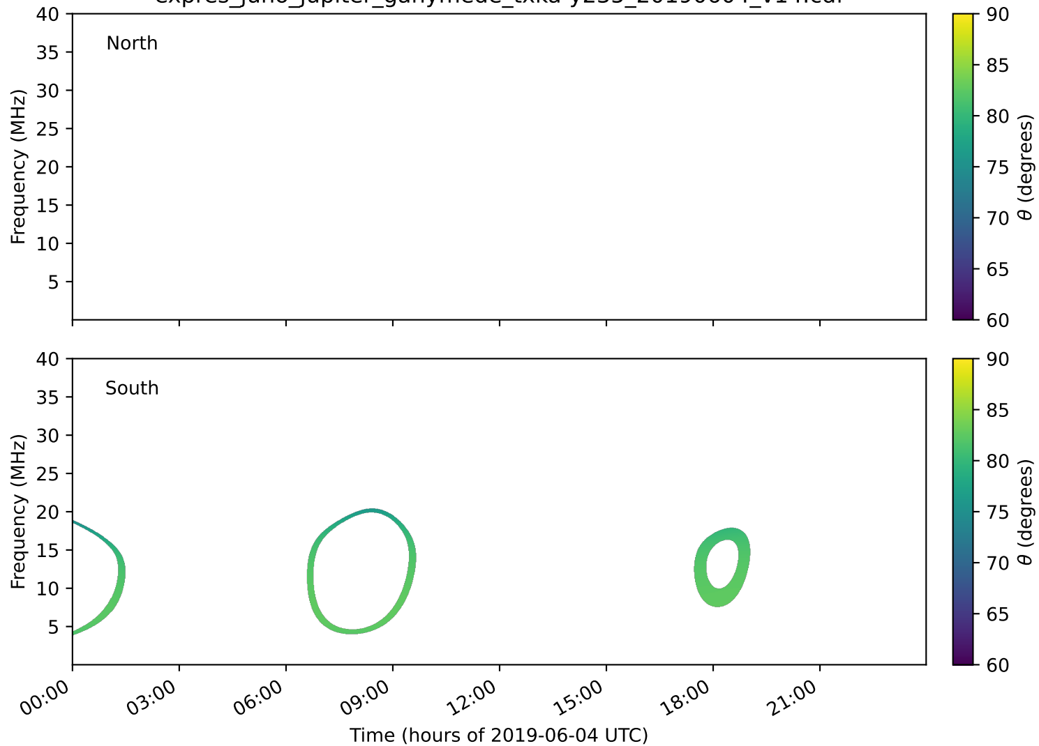
expres_juno_jupiter_ganymede_txka-y235_20190604_v14.cdf
