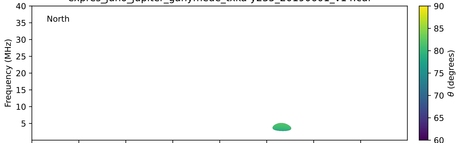
expres_juno_jupiter_ganymede_txka-y235_20190601_v14.cdf
