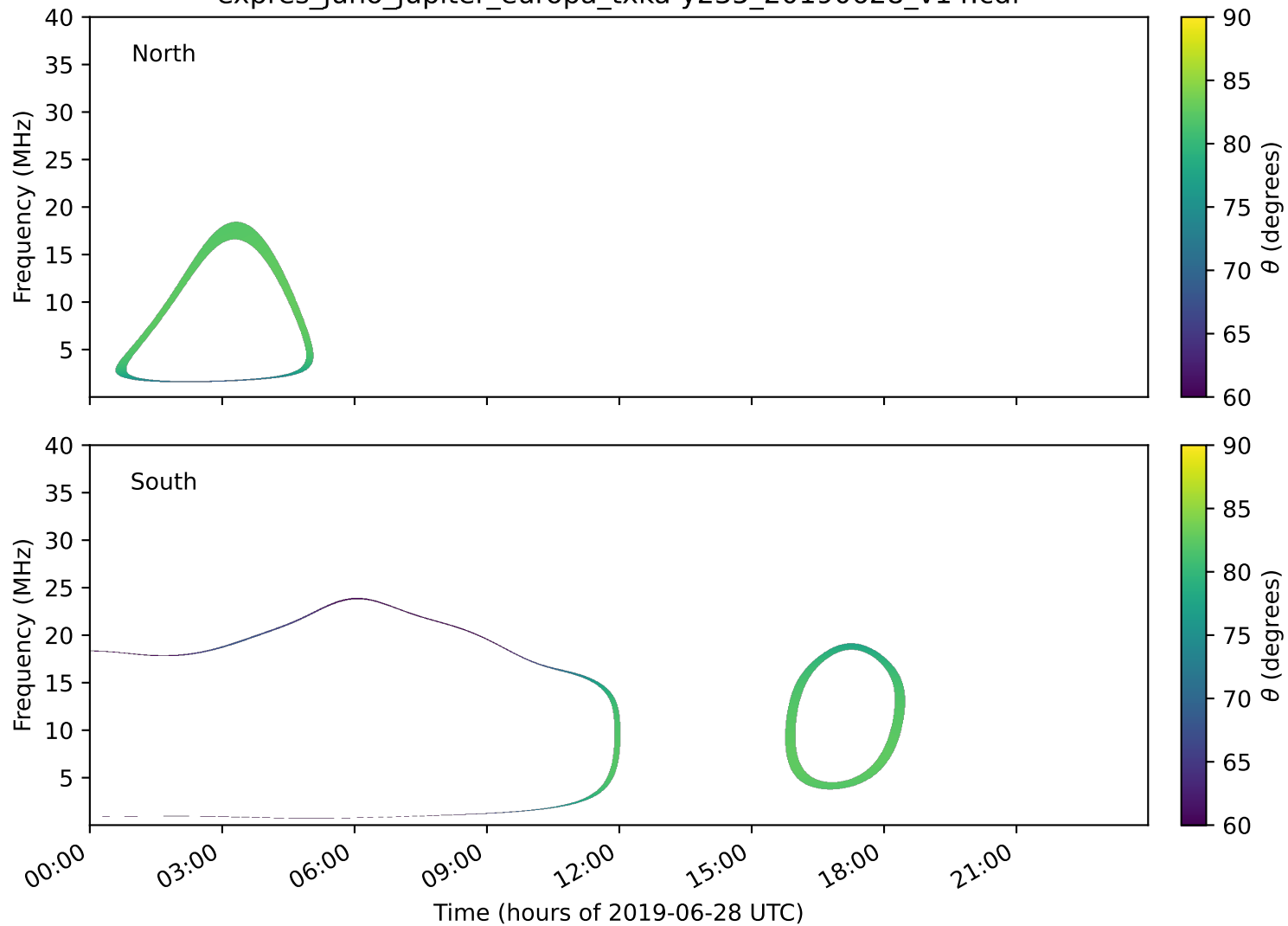
expres_juno_jupiter_europa_txka-y235_20190628_v14.cdf
