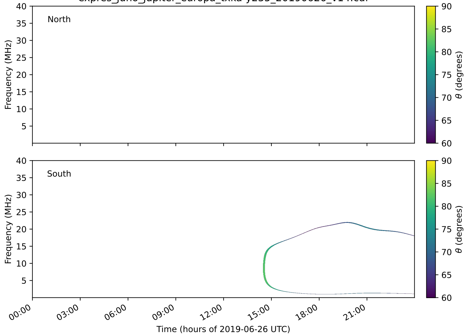
expres_juno_jupiter_europa_txka-y235_20190626_v14.cdf
