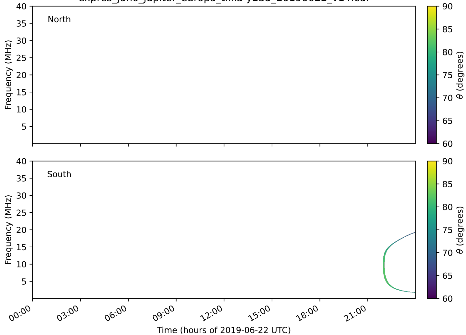
expres_juno_jupiter_europa_txka-y235_20190622_v14.cdf
