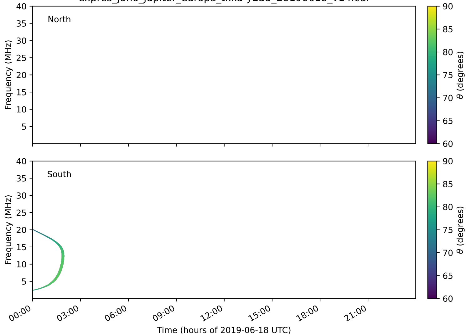
expres_juno_jupiter_europa_txka-y235_20190618_v14.cdf
