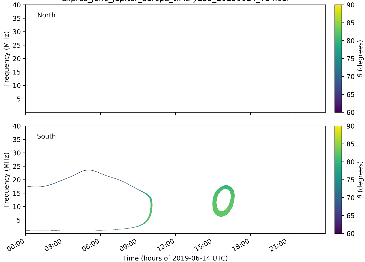
expres_juno_jupiter_europa_txka-y235_20190614_v14.cdf
