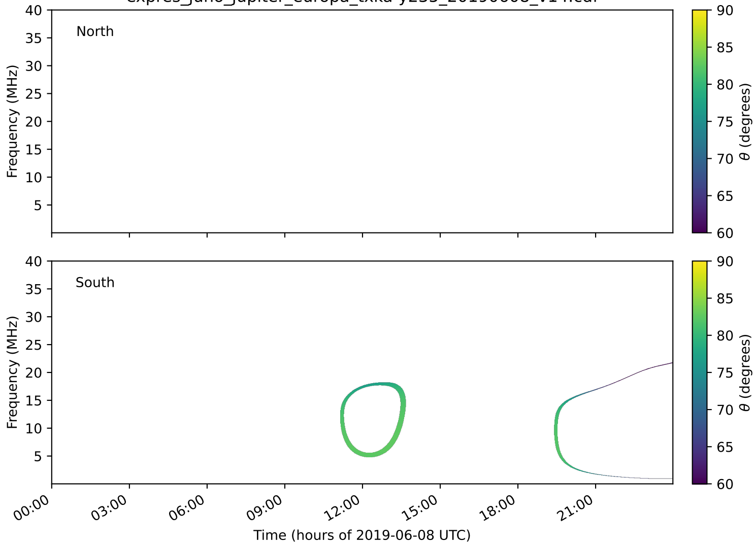
expres_juno_jupiter_europa_txka-y235_20190608_v14.cdf
