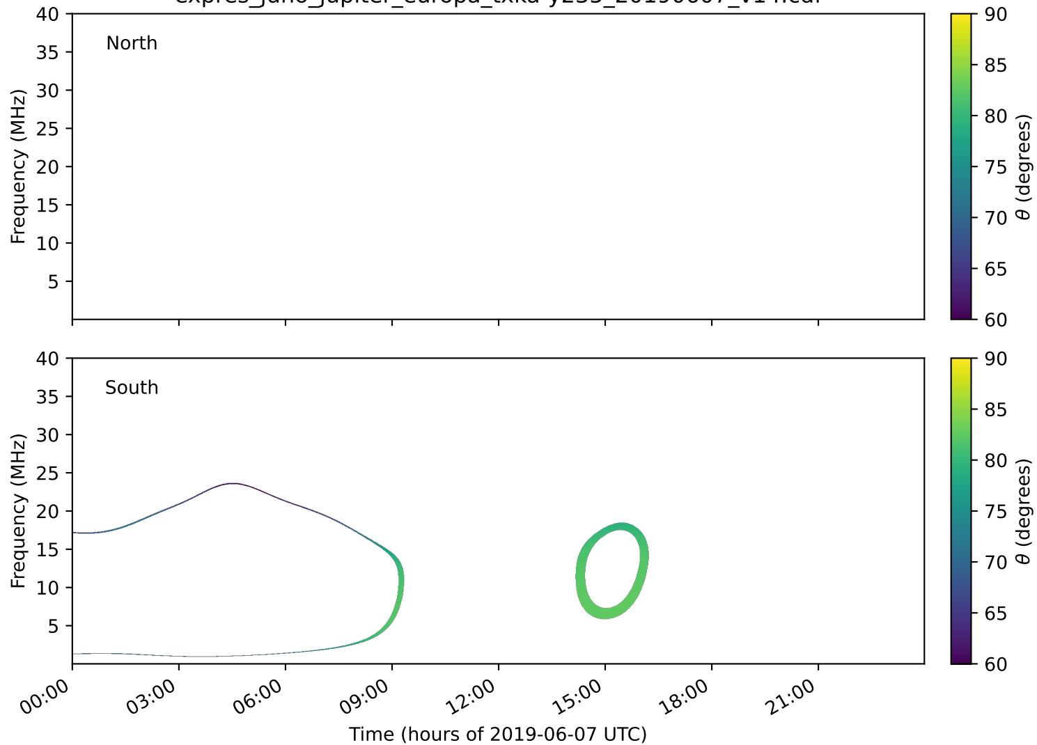
expres_juno_jupiter_europa_txka-y235_20190607_v14.cdf
