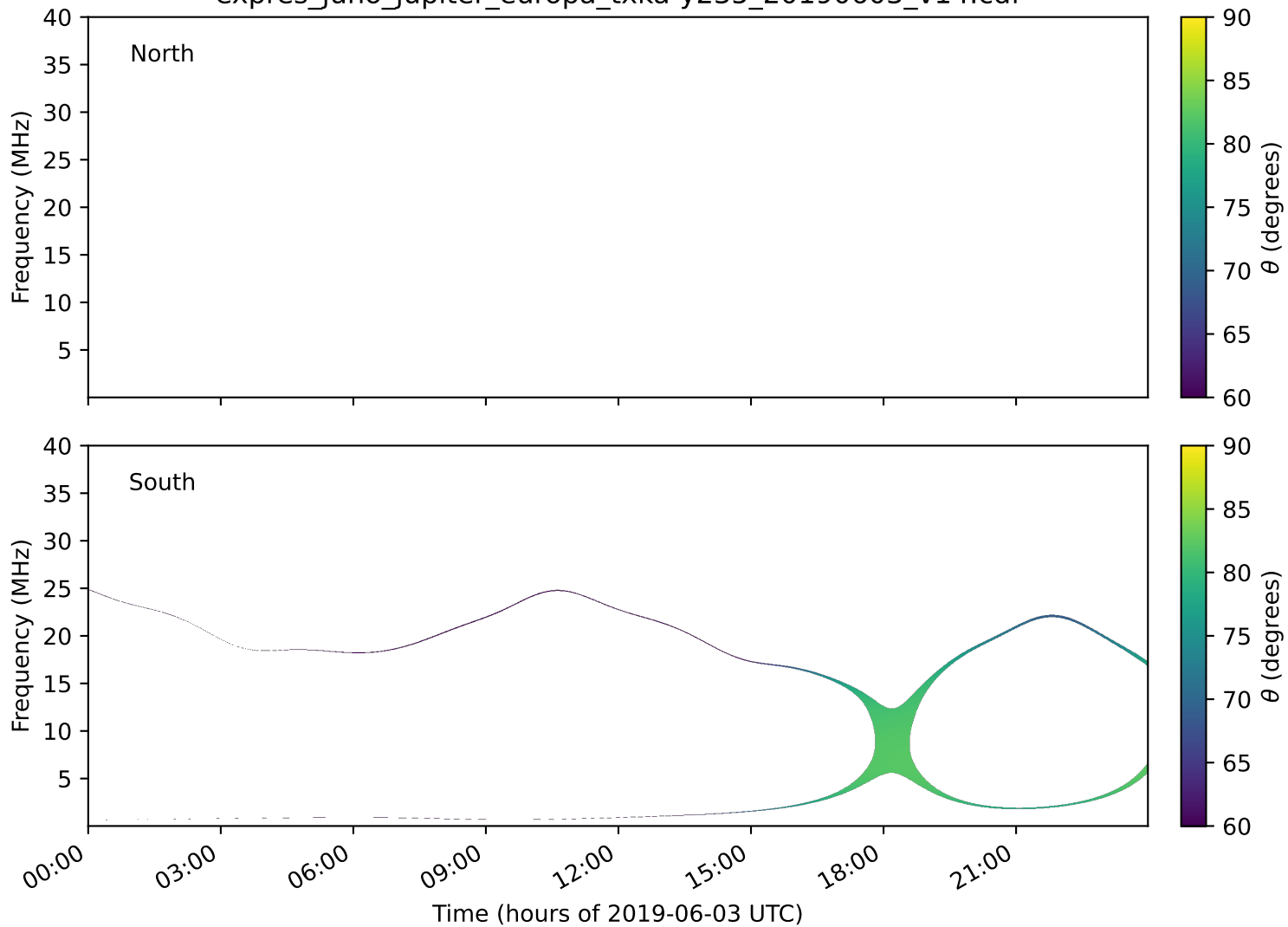
expres_juno_jupiter_europa_txka-y235_20190603_v14.cdf
