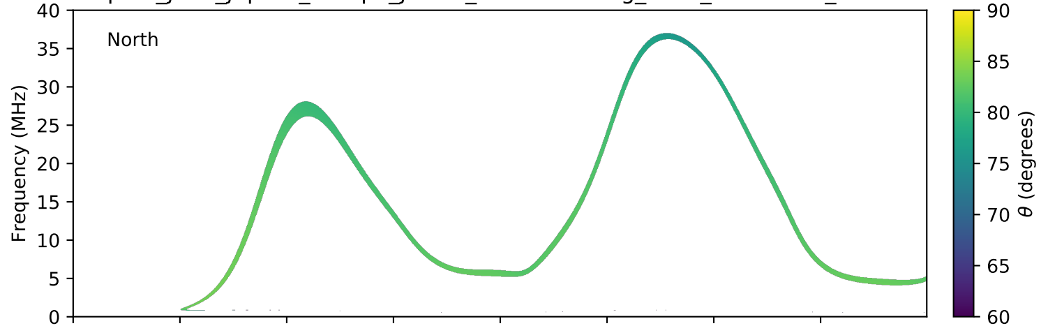
expres_juno_jupiter_europa_jrm09_lossc-wid1deg_3kev_20190627_v01.cdf
