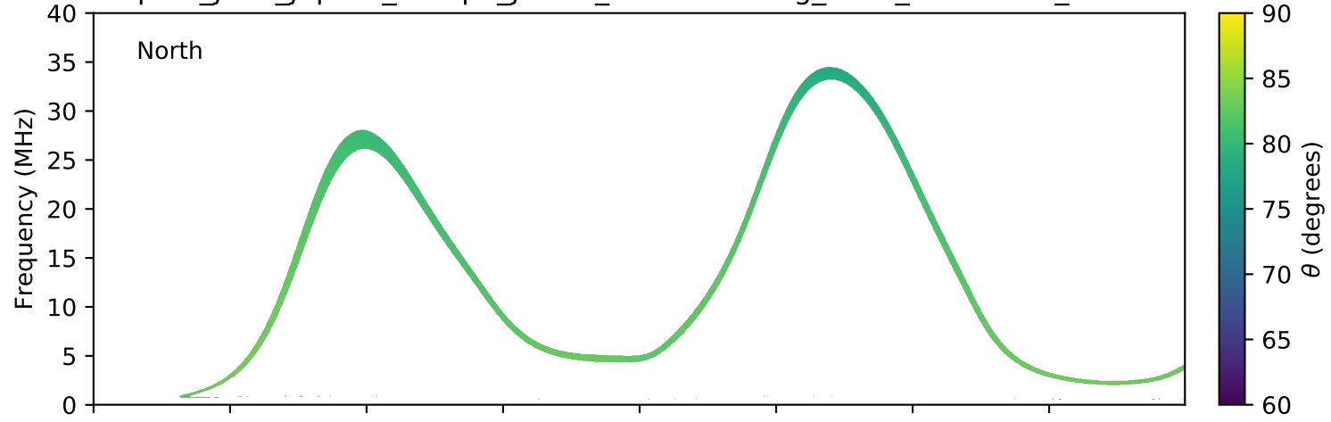
expres_juno_jupiter_europa_jrm09_lossc-wid1deg_3kev_20190620_v01.cdf
