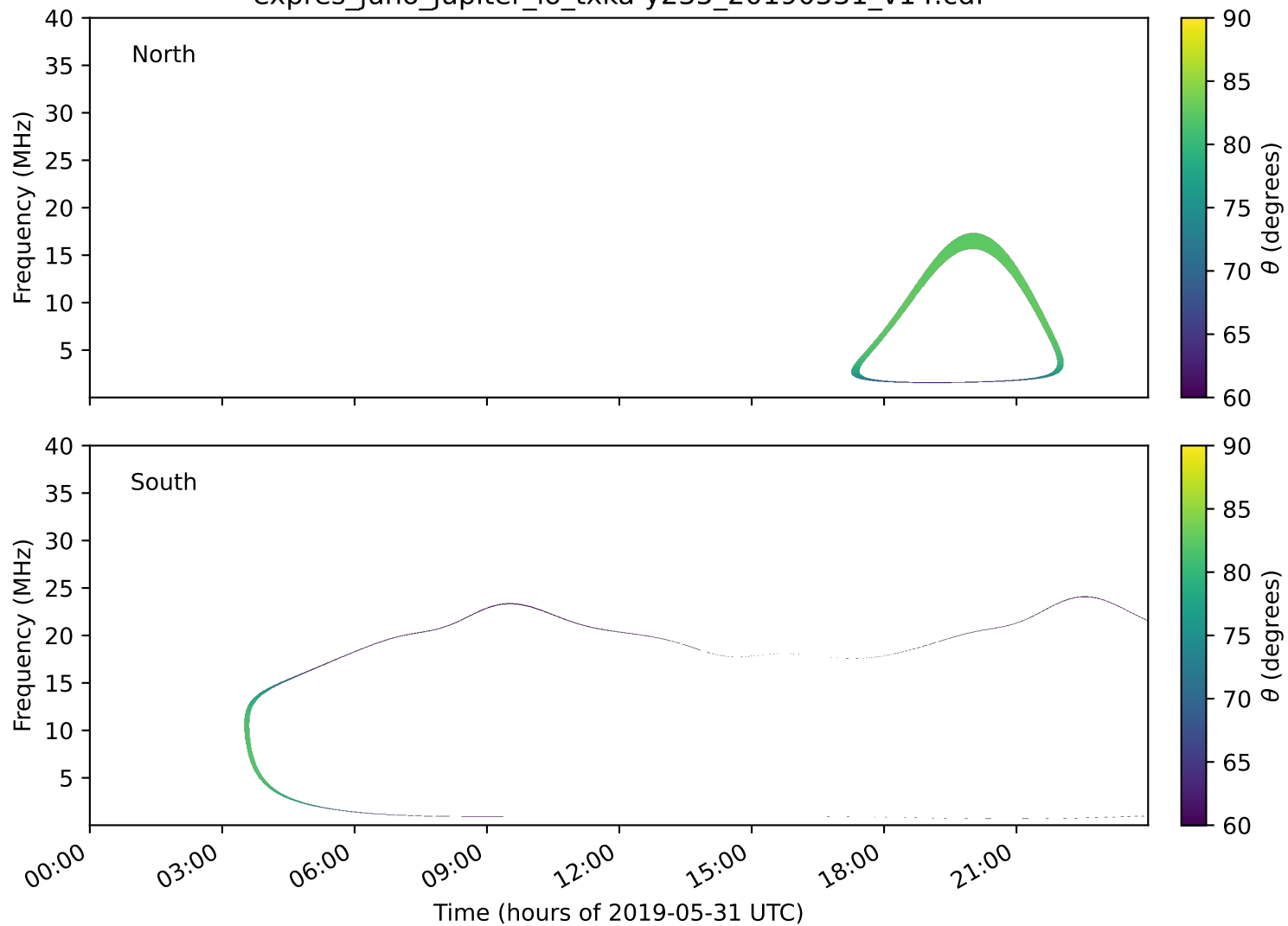
expres_juno_jupiter_io_txka-y235_20190531_v14.cdf
