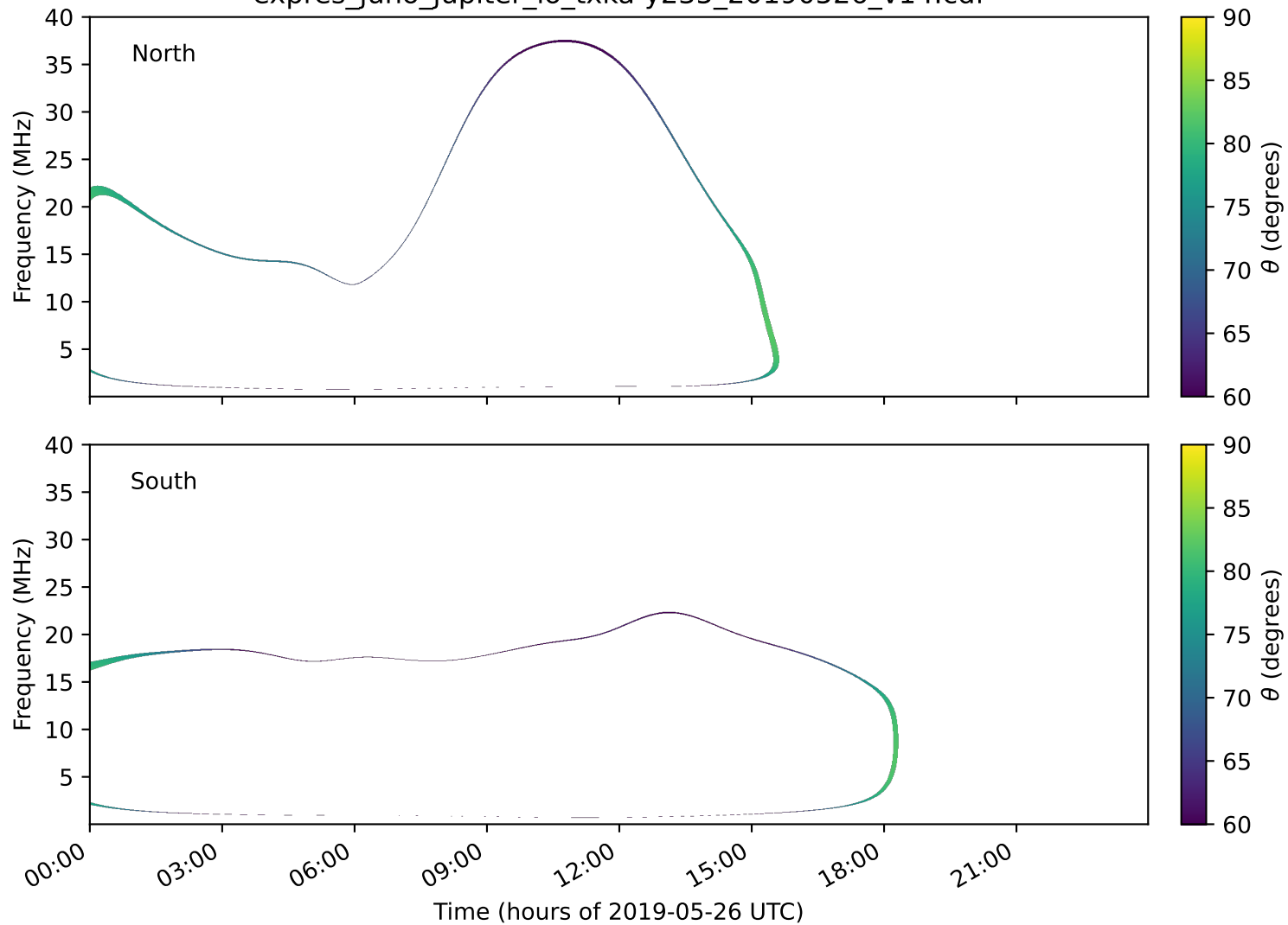
expres_juno_jupiter_io_txka-y235_20190526_v14.cdf
