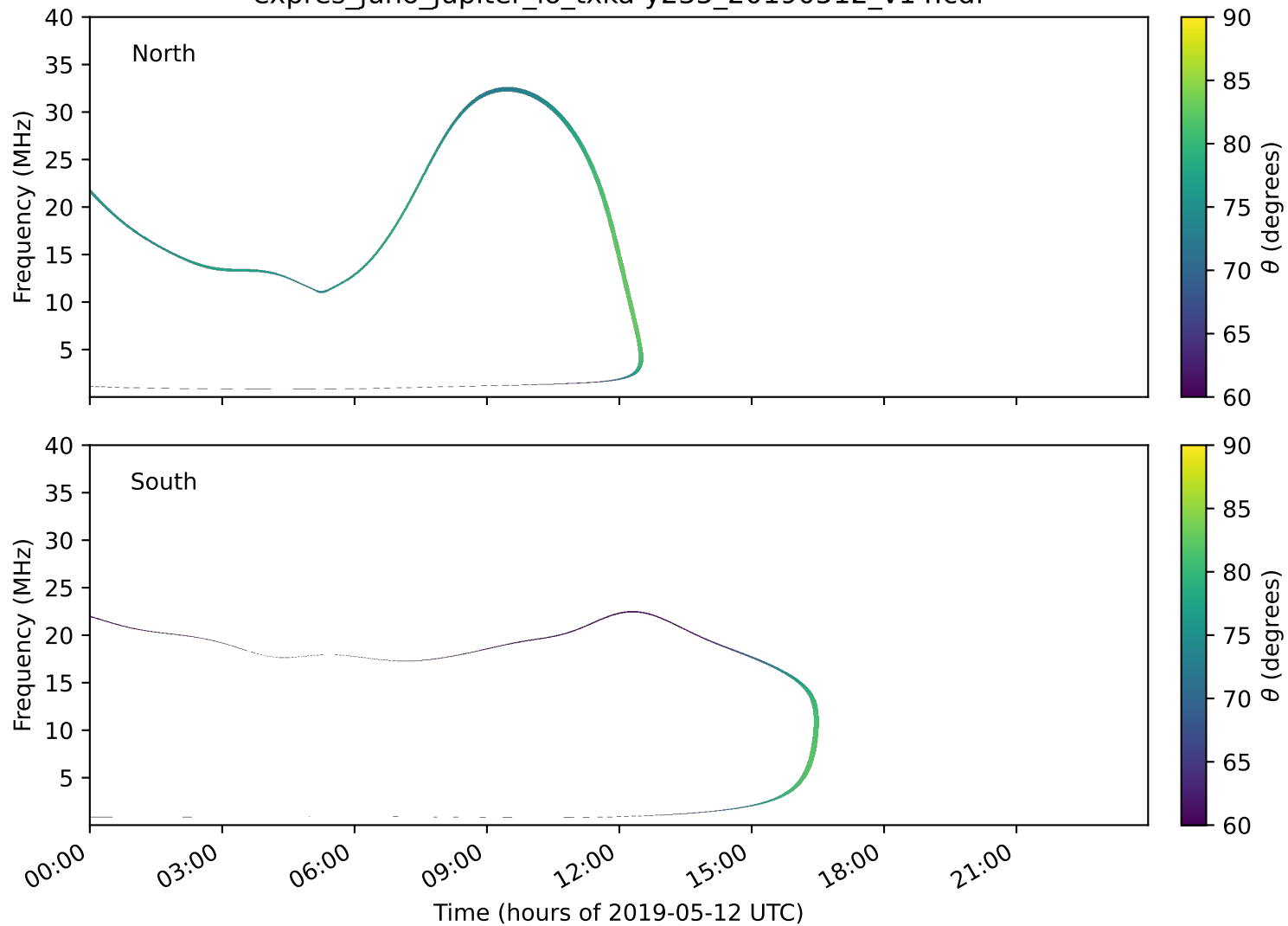
expres_juno_jupiter_io_txka-y235_20190512_v14.cdf
