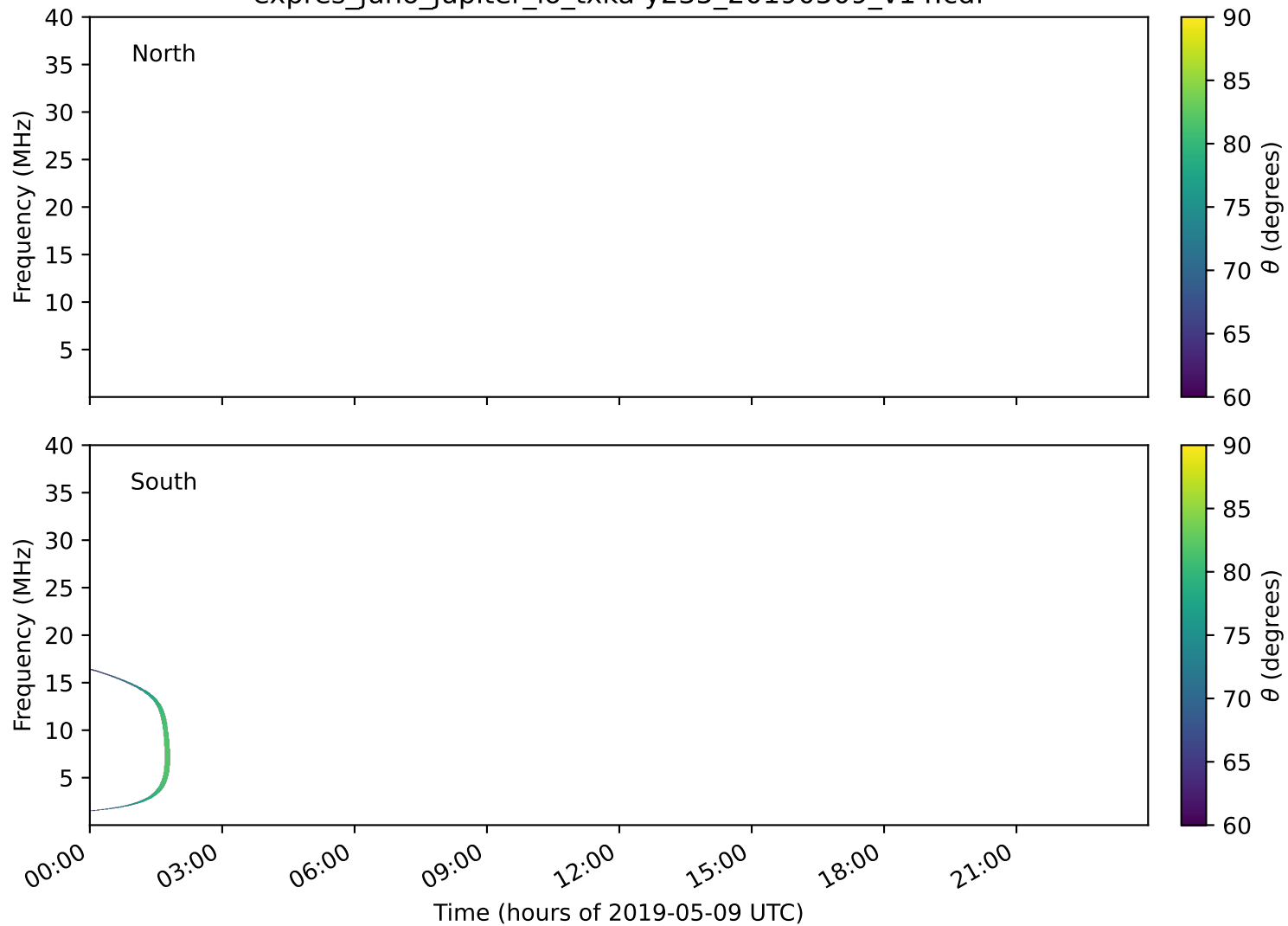
expres_juno_jupiter_io_txka-y235_20190509_v14.cdf
