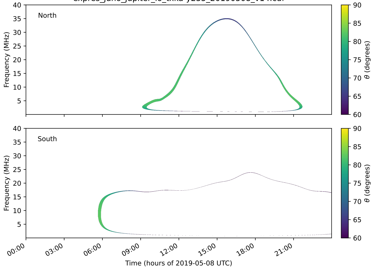
expres_juno_jupiter_io_txka-y235_20190508_v14.cdf
