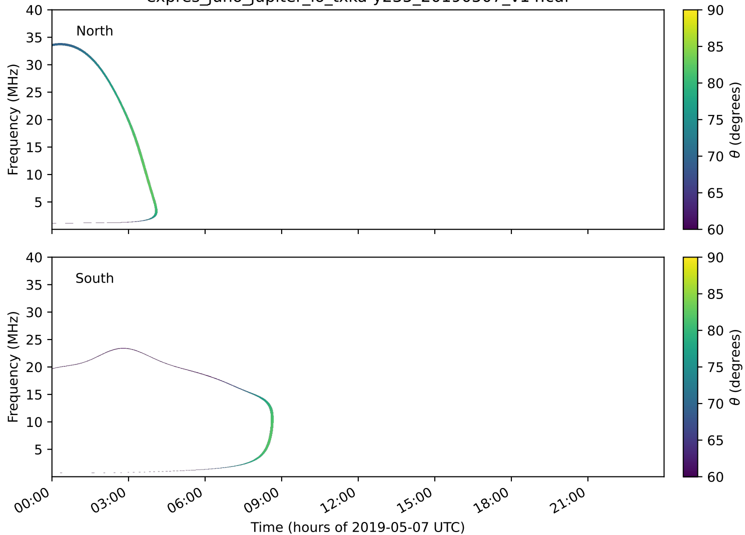
expres_juno_jupiter_io_txka-y235_20190507_v14.cdf
