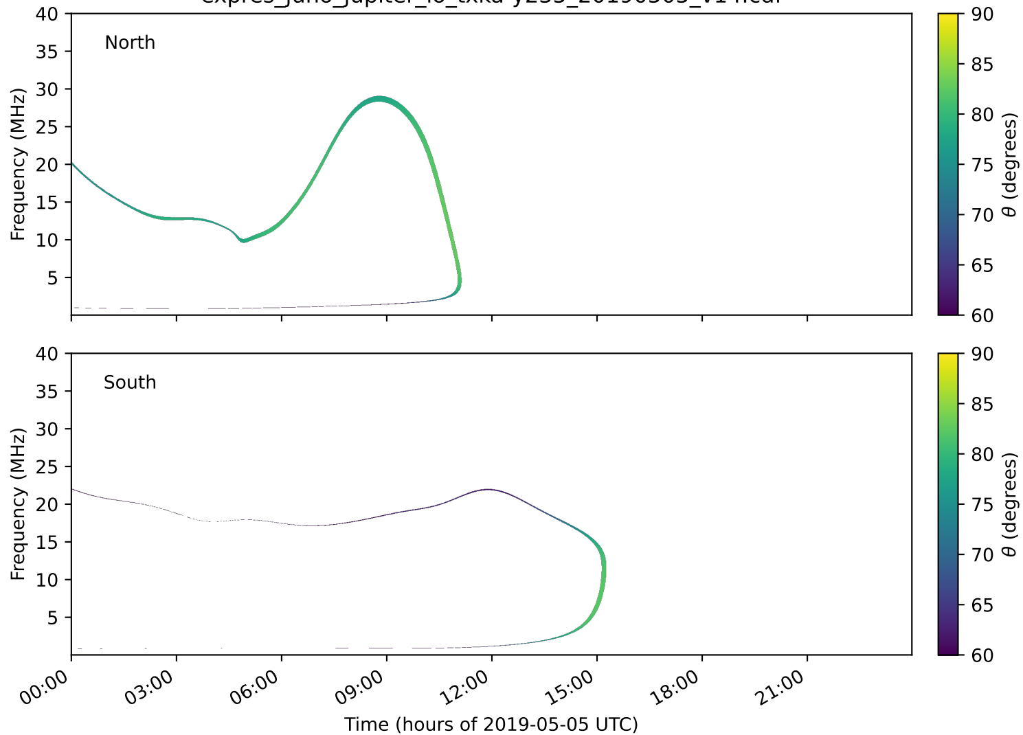
expres_juno_jupiter_io_txka-y235_20190505_v14.cdf
