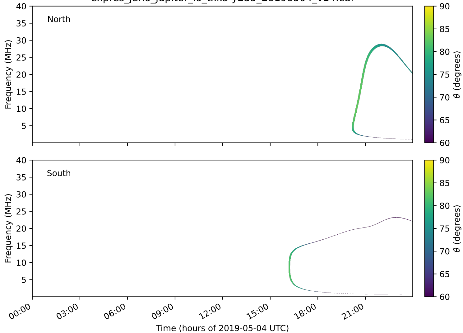
expres_juno_jupiter_io_txka-y235_20190504_v14.cdf
