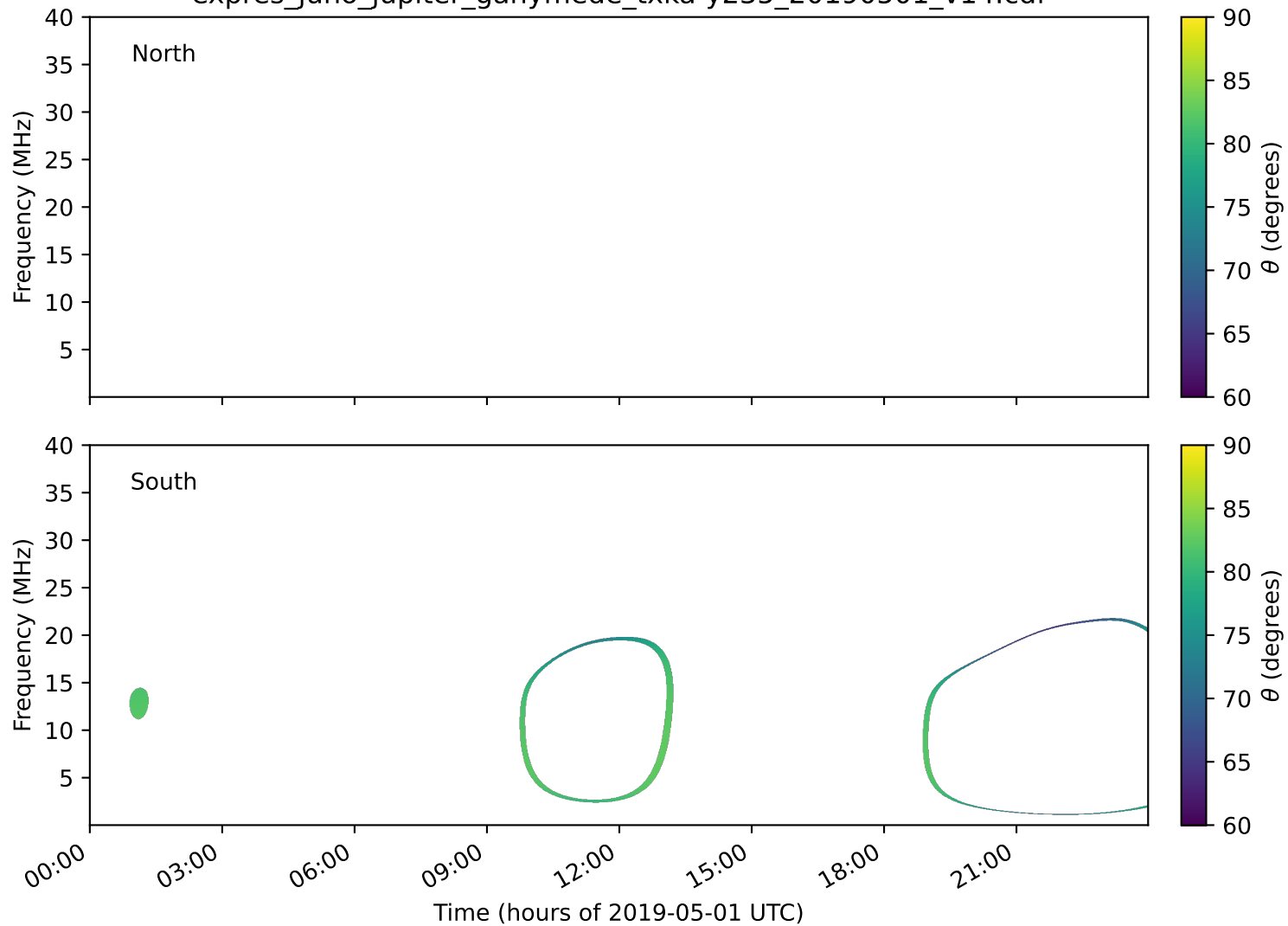
expres_juno_jupiter_ganymede_txka-y235_20190501_v14.cdf
