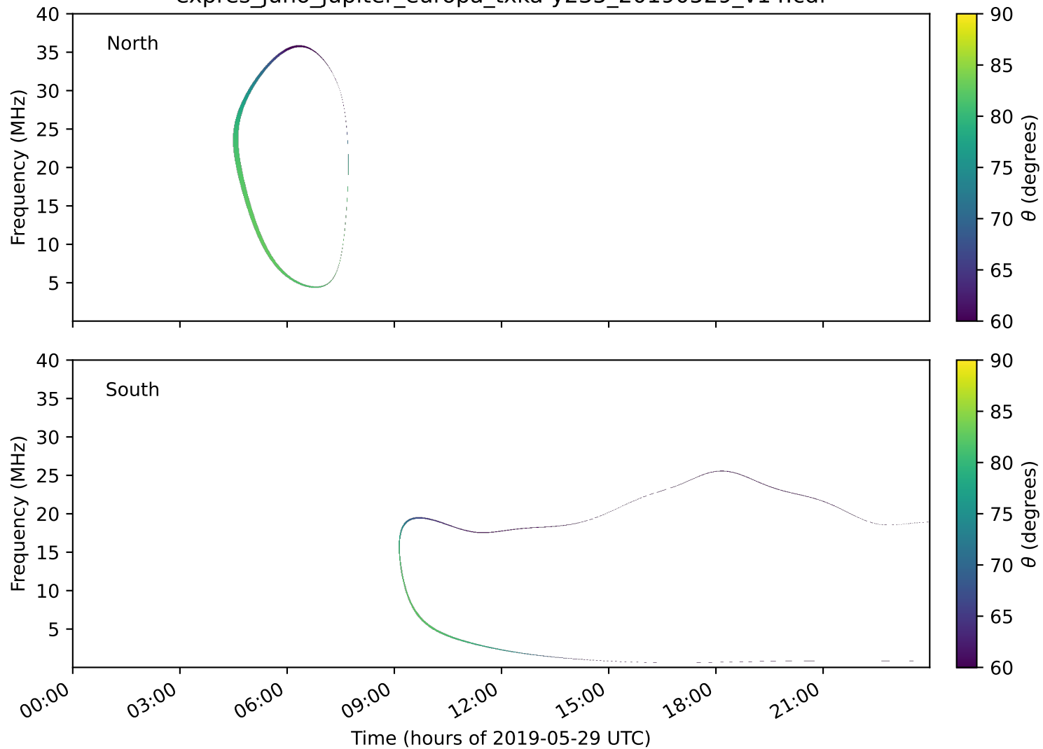
expres_juno_jupiter_europa_txka-y235_20190529_v14.cdf
