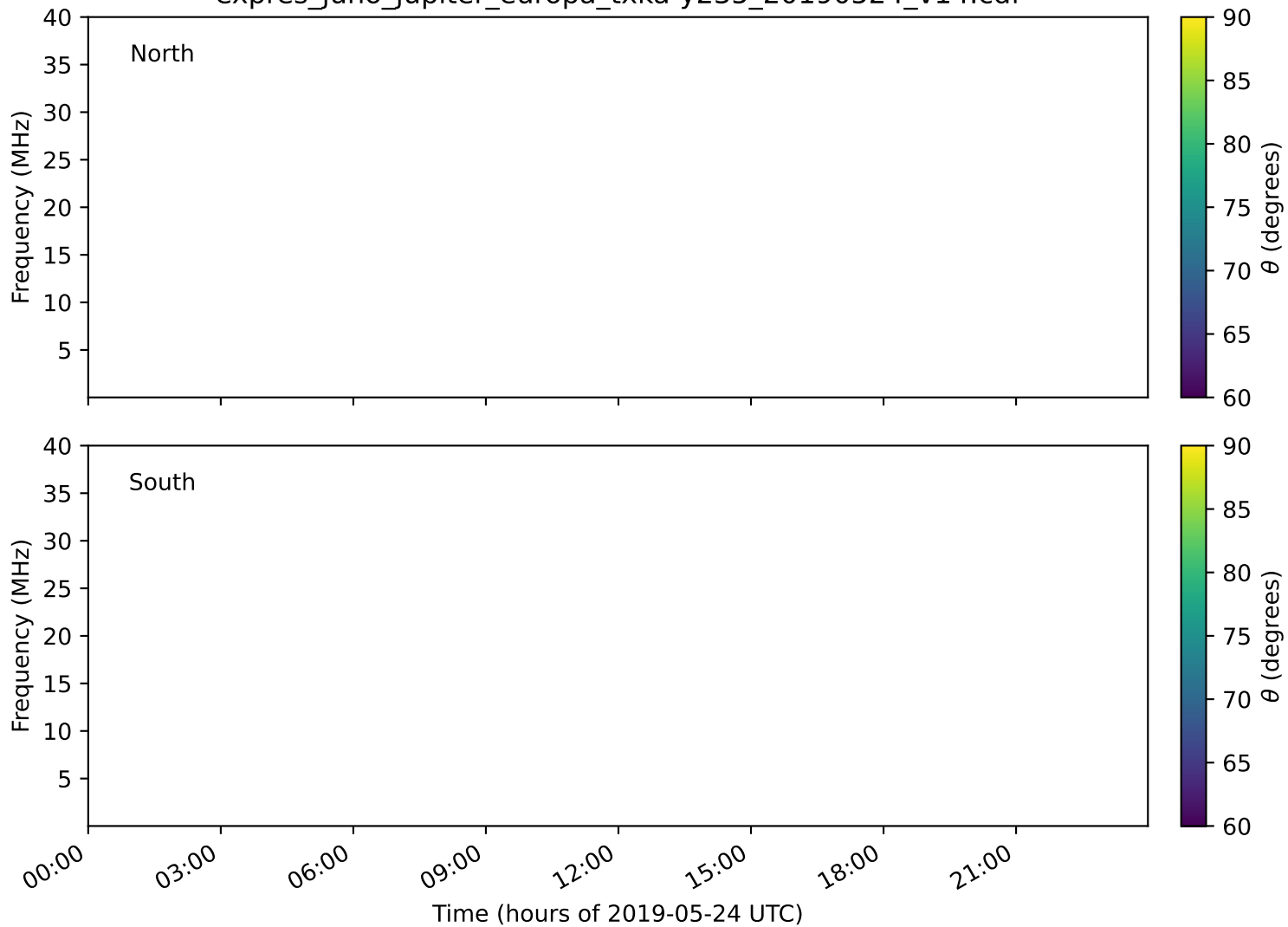
expres_juno_jupiter_europa_txka-y235_20190524_v14.cdf
