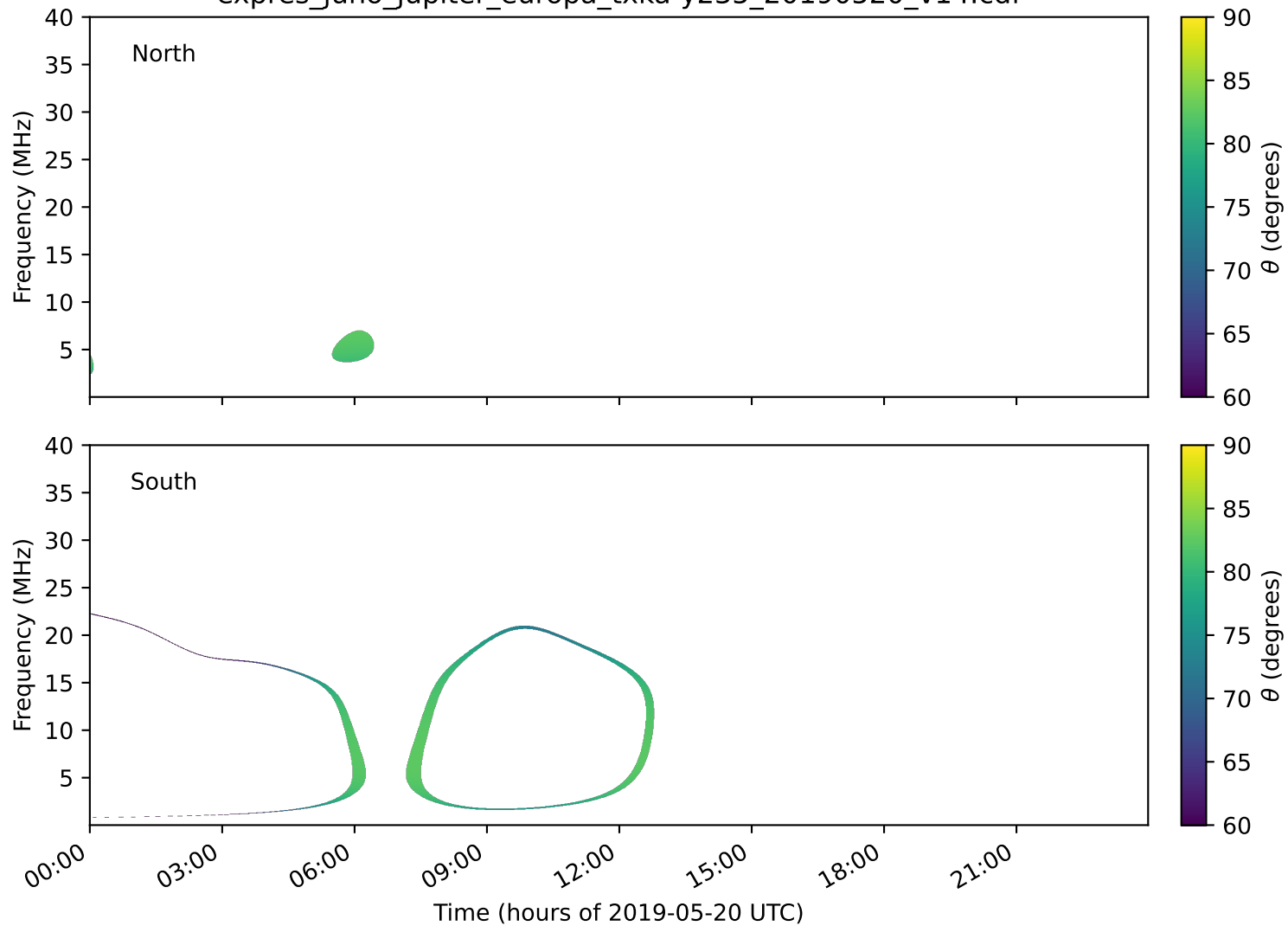
expres_juno_jupiter_europa_txka-y235_20190520_v14.cdf
