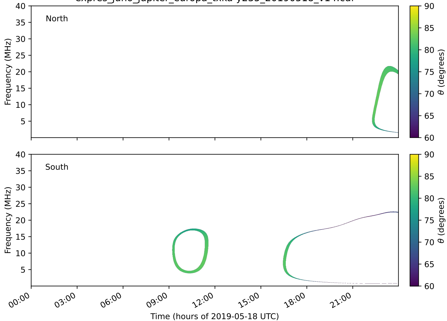
expres_juno_jupiter_europa_txka-y235_20190518_v14.cdf
