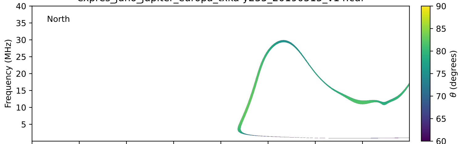
expres_juno_jupiter_europa_txka-y235_20190515_v14.cdf
